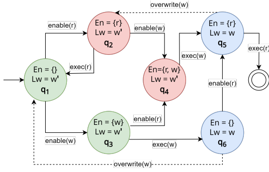
(a) Scheduling a positive constraint w \not\leq^r r . Blue states prioritize r and deprioritize any write other than w . Red states prioritize w and deprioritize r . Green states represent no prioritization.
