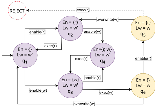
(b) Scheduling a negative constraint w \geq r . Purple states prioritize r and deprioritize w . Yellow states prioritize all writes apart from w and deprioritize r .
